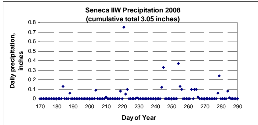
Figure 7. Ambient rainfall at the IIW study site.
