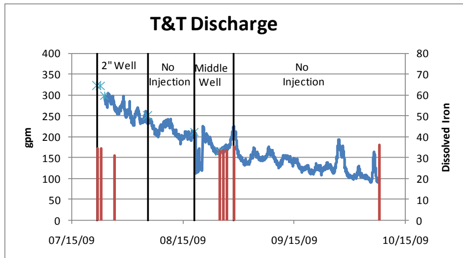
Figure 9. Dissolved iron at the T&T discharge
