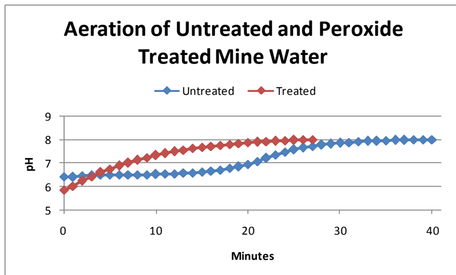
Figure 6. Comparative aeration test.
