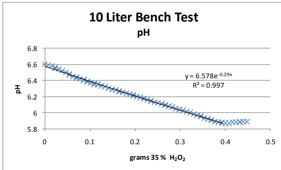
Figure 4. Change in pH with the addition of \text{H}_2\text{O}_2
