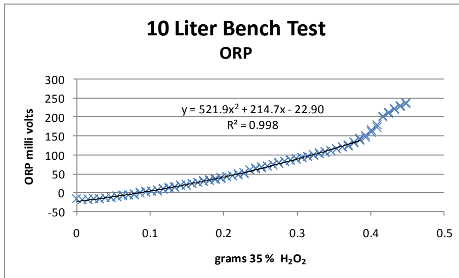
Figure 5. Change in ORP with the addition of \text{H}_2\text{O}_2
