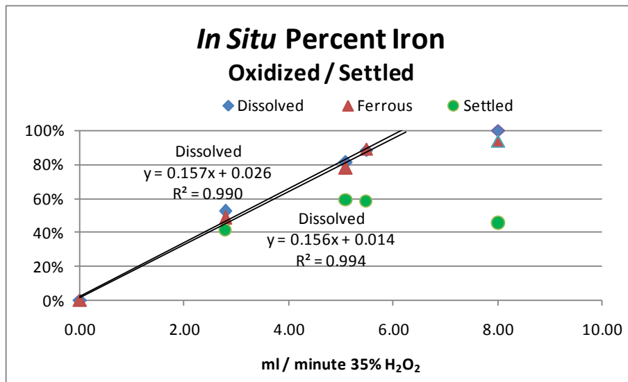
Figure 7. In Situ Iron oxidation and settlement.
