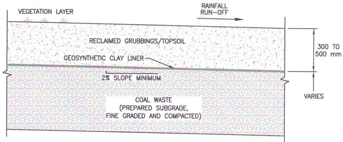
Figure 3.1 Capping Detail
