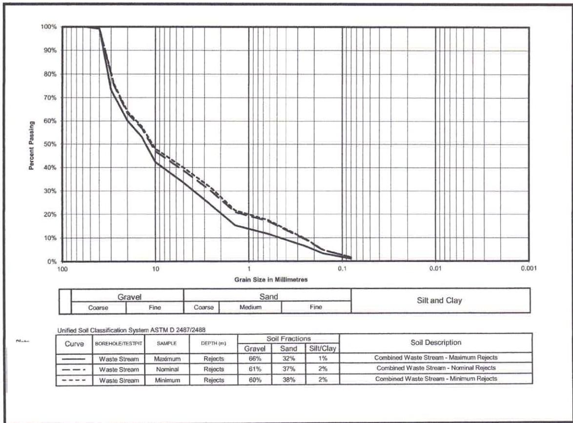
Figure 2.4 Grain Size Distribution of Waste Streams
