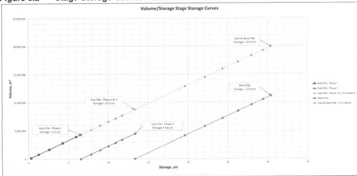
Figure 3.2 Stage Storage Curves - Volume vs. Time
