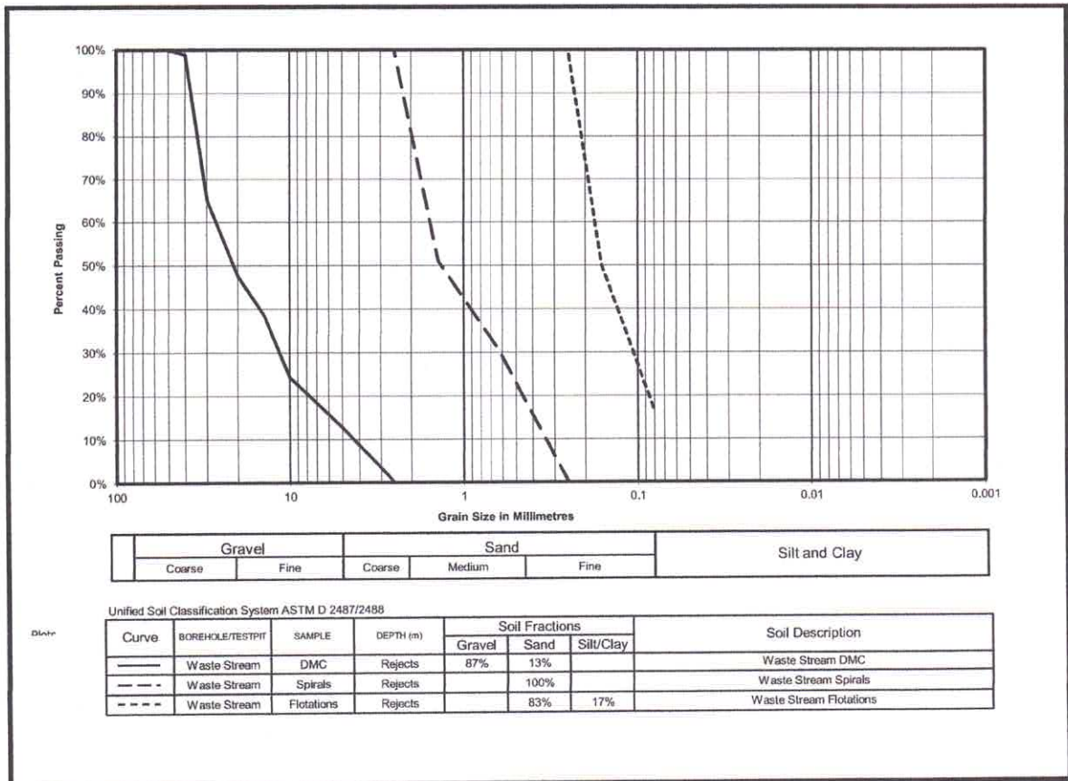
Figure 2.2 Grain Size Distribution of WasteStreams
