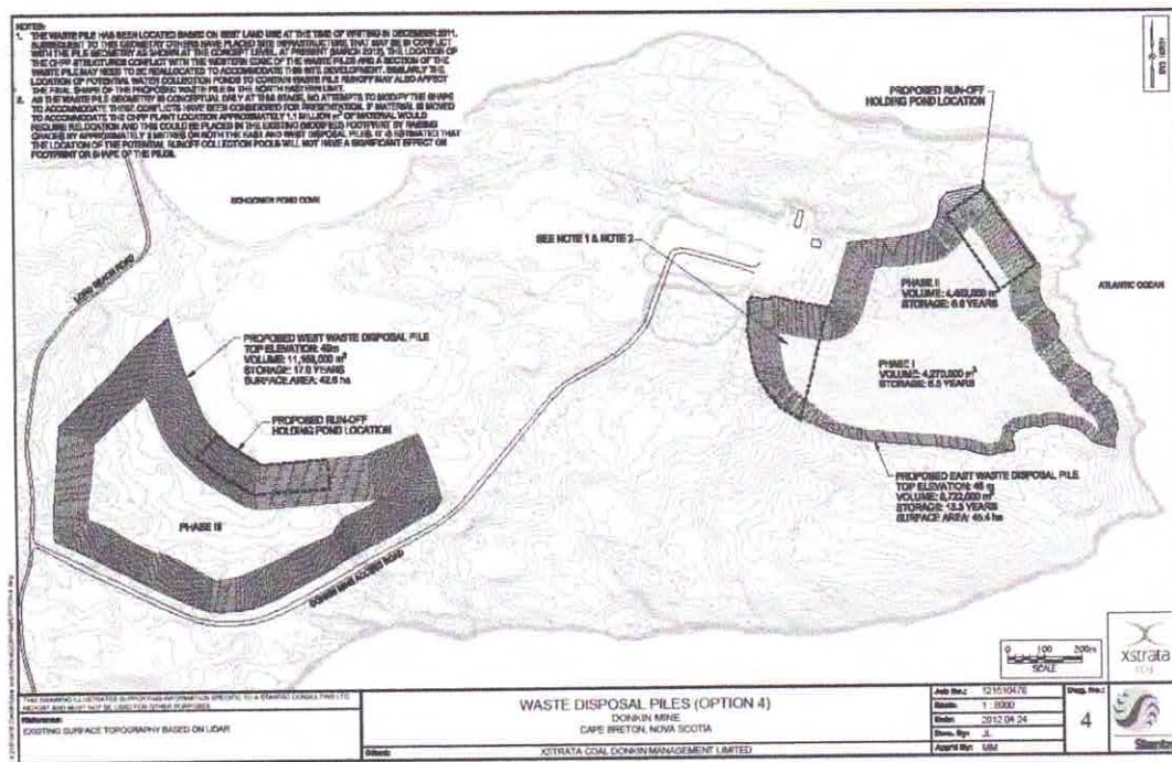
Drawing 3.4 Disposal Option 4
