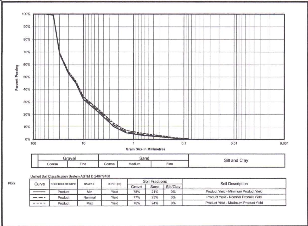
Figure 2.3 Grain Size Distribution of Product Streams
