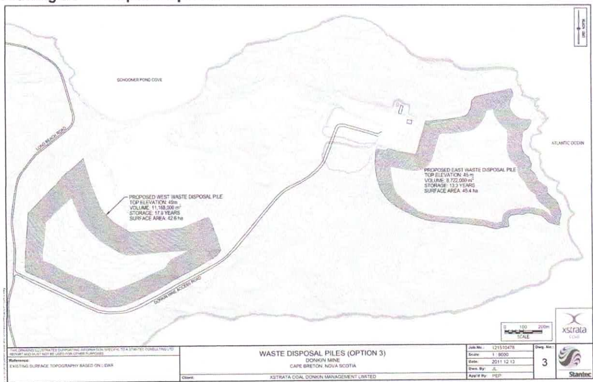
Drawing 3.3 Disposal Option 3
